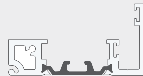
STACKING AND POCKET MID-HEIGHT SILL 1-1/2"
